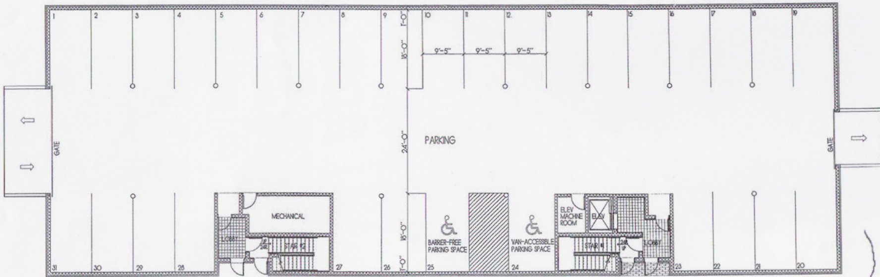
Ground Floor / Parking
